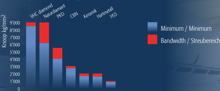
Hardness Comparison (Knoop kg/mm 2 ) Härtevergleich (Knoop kg/mm 2 )
